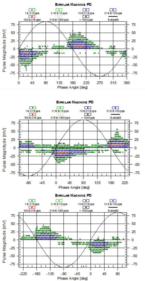
Fig. 1: Phase-resolved PD plots for 3 phases using 80 pF capacitive sensors on a generator operating at 18 kV, 117 MW and 200 kPag. The horizontal scale is the phase angle of the power frequency. The vertical scale is the PD magnitude in mV. The color of the dots represents the PD pulse repetition rate.
