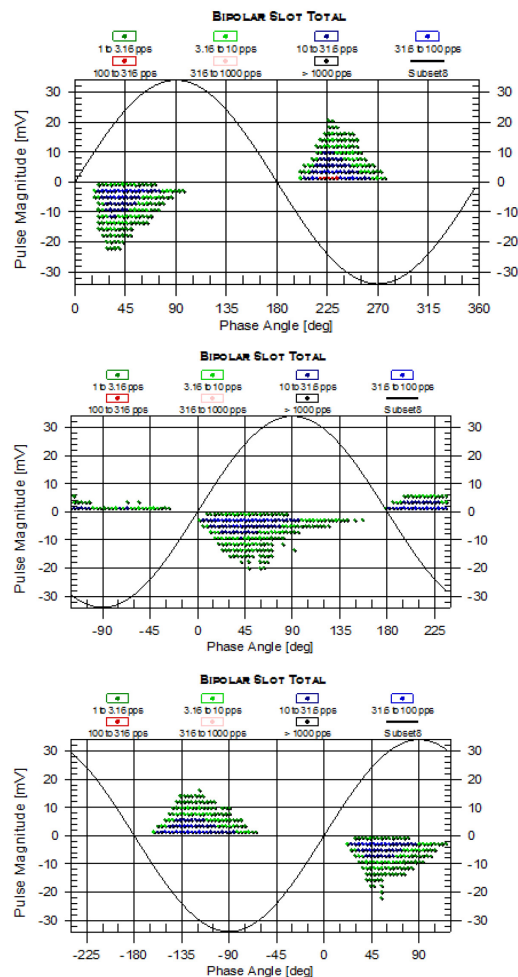
Fig. 2: PD plots using antennae sensors from a generator operating at 24 kV, 467 MW and 410 kPag. The data from phases A, B and C (top to bottom) are phase shifted to reveal any phase-to-phase PD in the endwinding.
