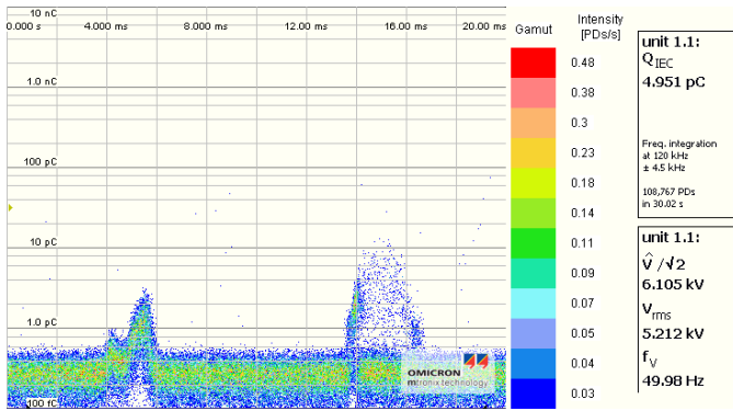
Fig. 3. Measurement of a protrusion at the inner conductor at low level according to IEC
