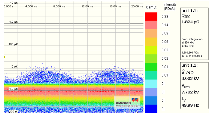
Fig. 1. Measurement of moving particle accordance with IEC
