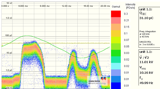
Fig. 5. Measurement of a protrusion on an inner conductor at higher level according to IEC
